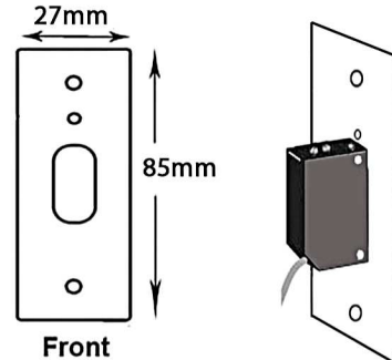
Flush mount (sensor inside hollow wall) Bracket standard in white or black
